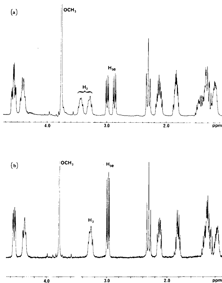
Figure 1. 360 MHz ^1\text{H} nmr spectra in perdeuteriobenzene ( ca. 0.01 M ) of (+)- R - \alpha -methoxy- \alpha -(trifluoromethyl)-phenylacetic acid [(+)-Mosher's acid; (+)-MTPA] and (a) ( \pm )- 1 ; (b) ( \pm )- 1 from its diastereomeric salt with (+)- 2 , [\alpha]_D^{26} - 101.4^\circ . There is a 1:1 ratio between the amine substrate and Mosher's acid. Minimum detection limits by electronic integration of H_3 or H_{5e} were determined to be 1%.
